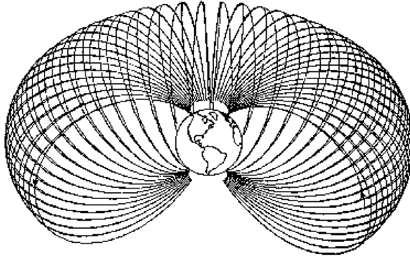
Figure 4: Typical trajectory of a charged particle in the Earth's magnetosphere, excluding gyromotion.
