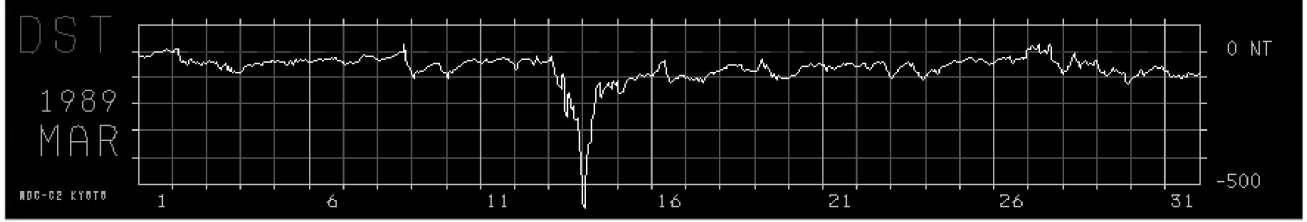
Figure 5: Dst data for March 1989 showing an exceptionally severe geomagnetic storm on the 13th.
