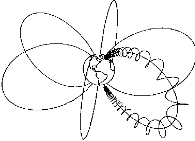
Figure 3: A typical trajectory of a charged particle trapped in the Earth’s magnetic field.
