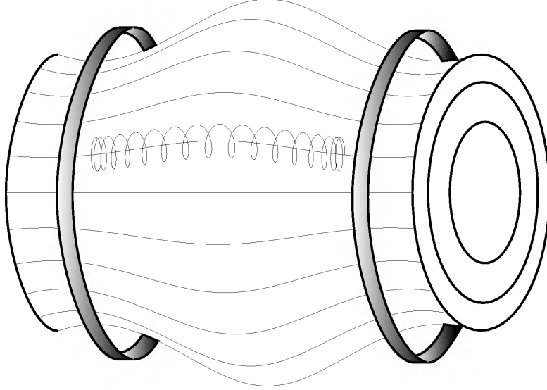
Figure 1: Motion of a trapped particle in a mirror machine.
