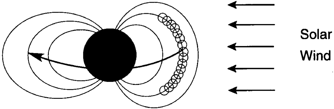
Figure 6: The distortion of the Earth's magnetic field by the solar wind.
